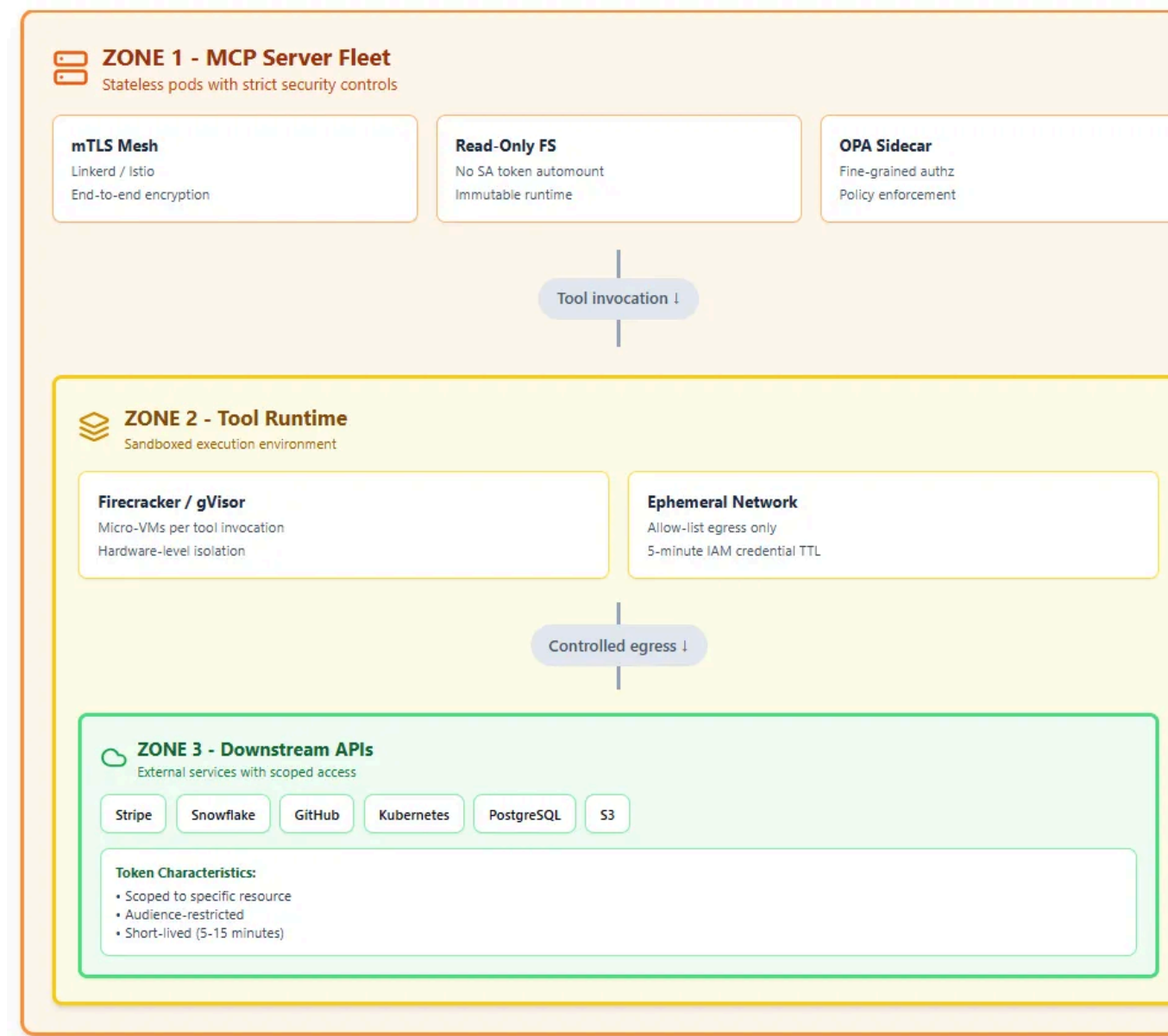
Figure 2: Three zones for MCP Server Architectures
